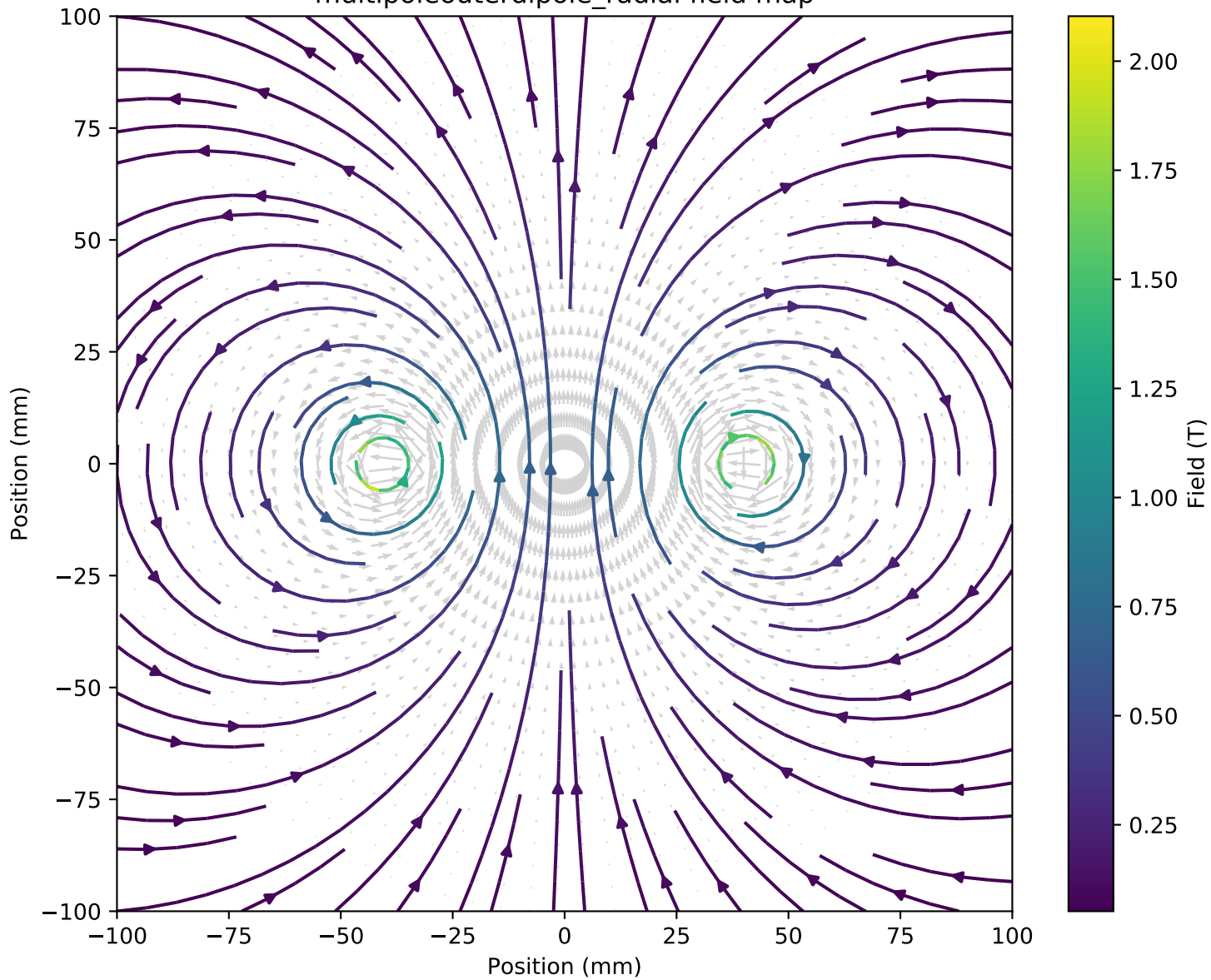
multipoleouterdipole_radial field map
