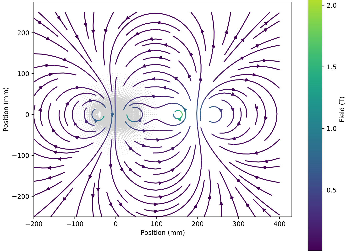
multipoleouterdipolelhc_radial field map
