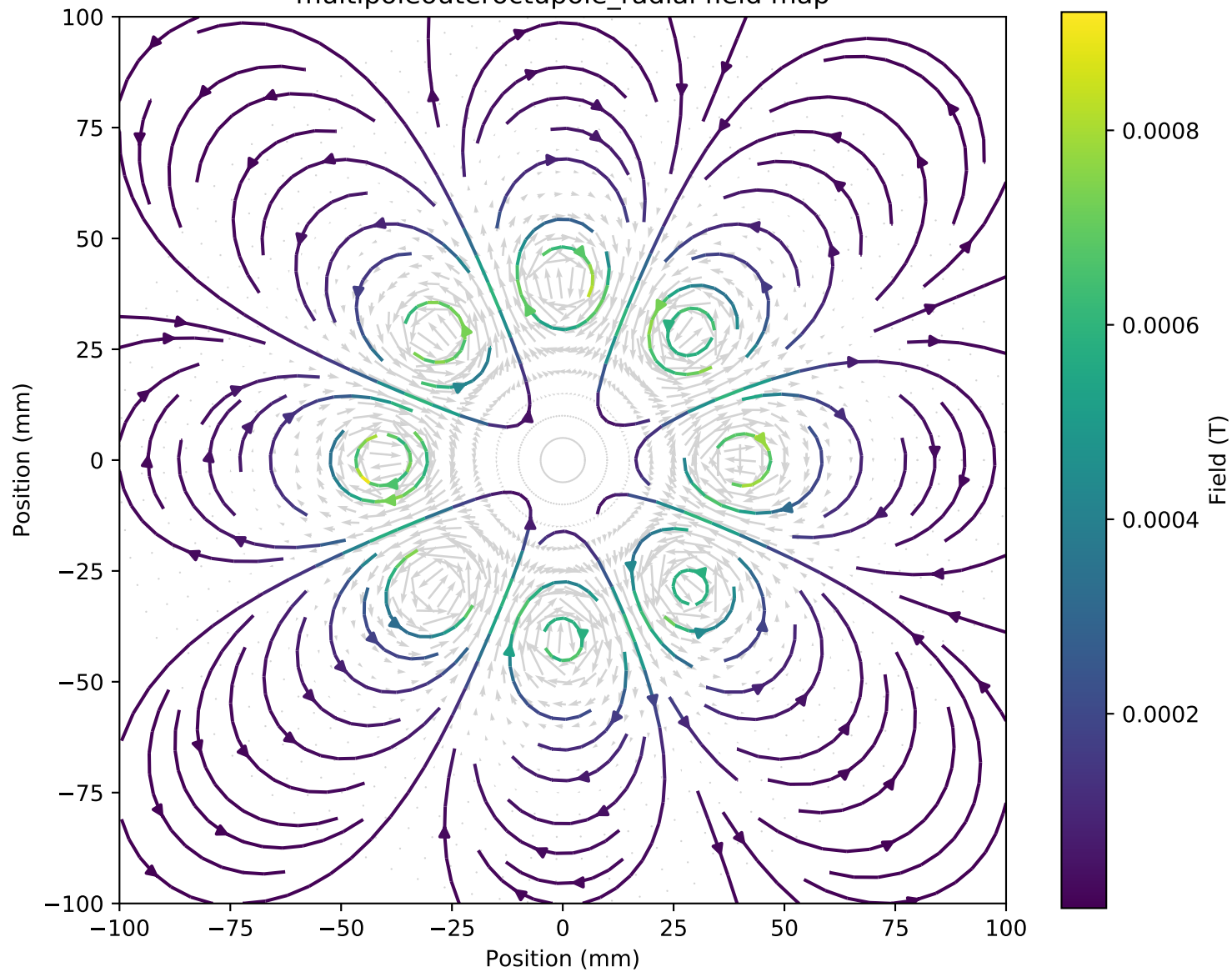
multipoleouteroctupole_radial field map
