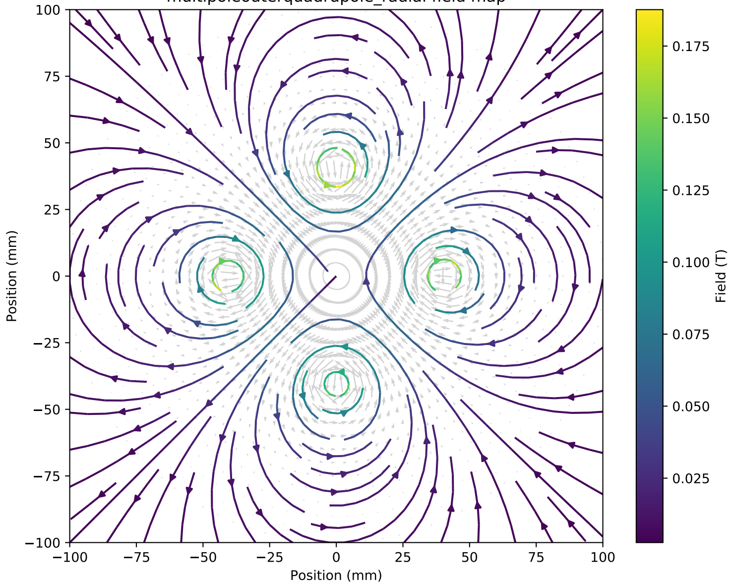
multipoleouterquadrupole_radial field map
