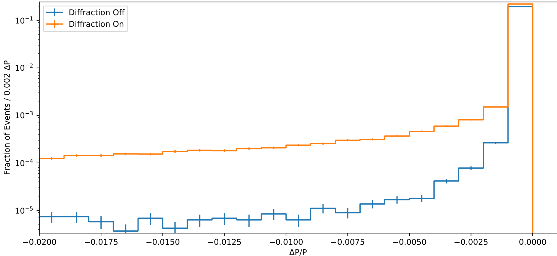
Proton Diffraction on Target of 40cm G4_C
