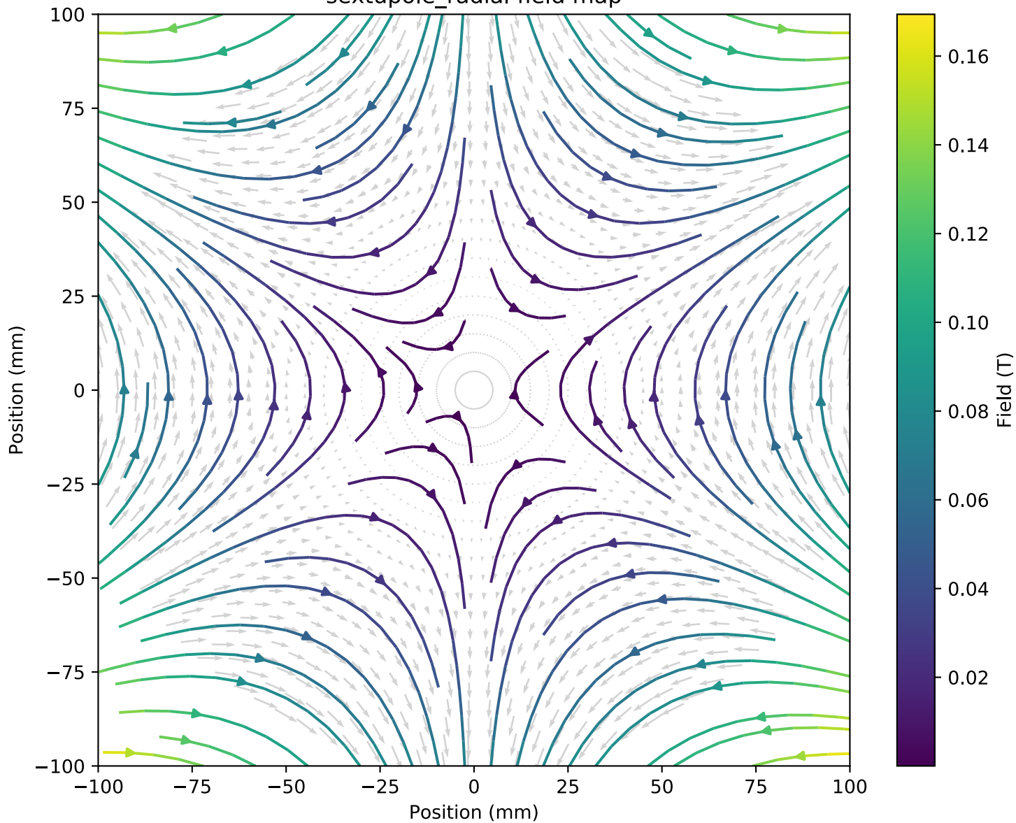
sextupole_radial field map
