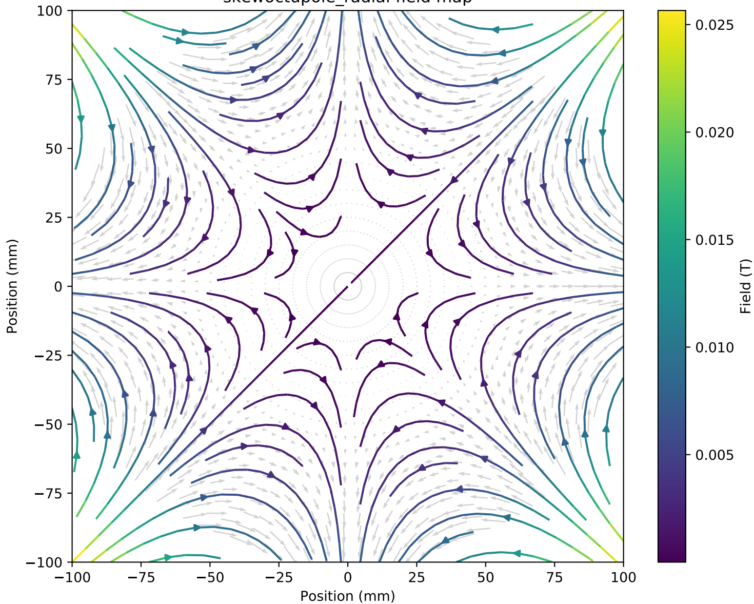
skewoctupole_radial field map
