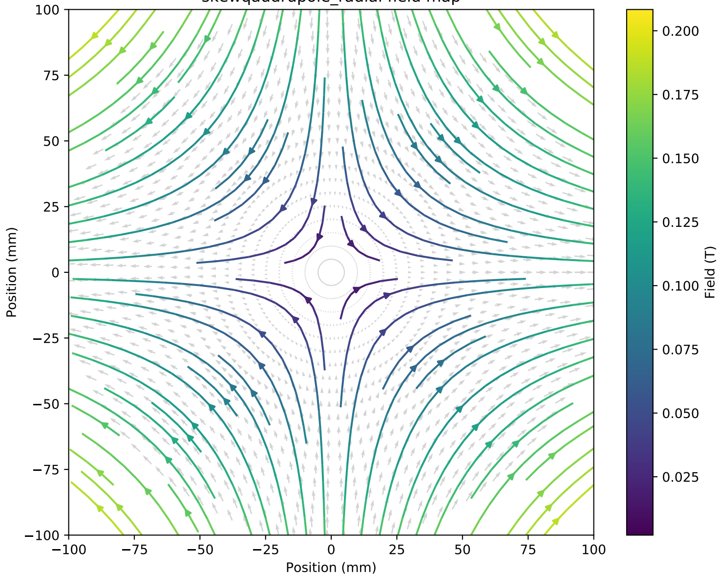
skewquadropole_radial field map
