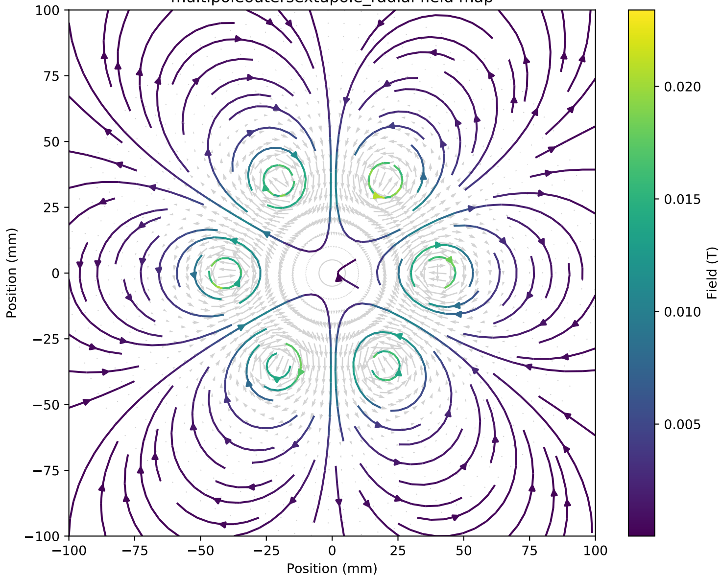
multipoleoutersextupole_radial field map
