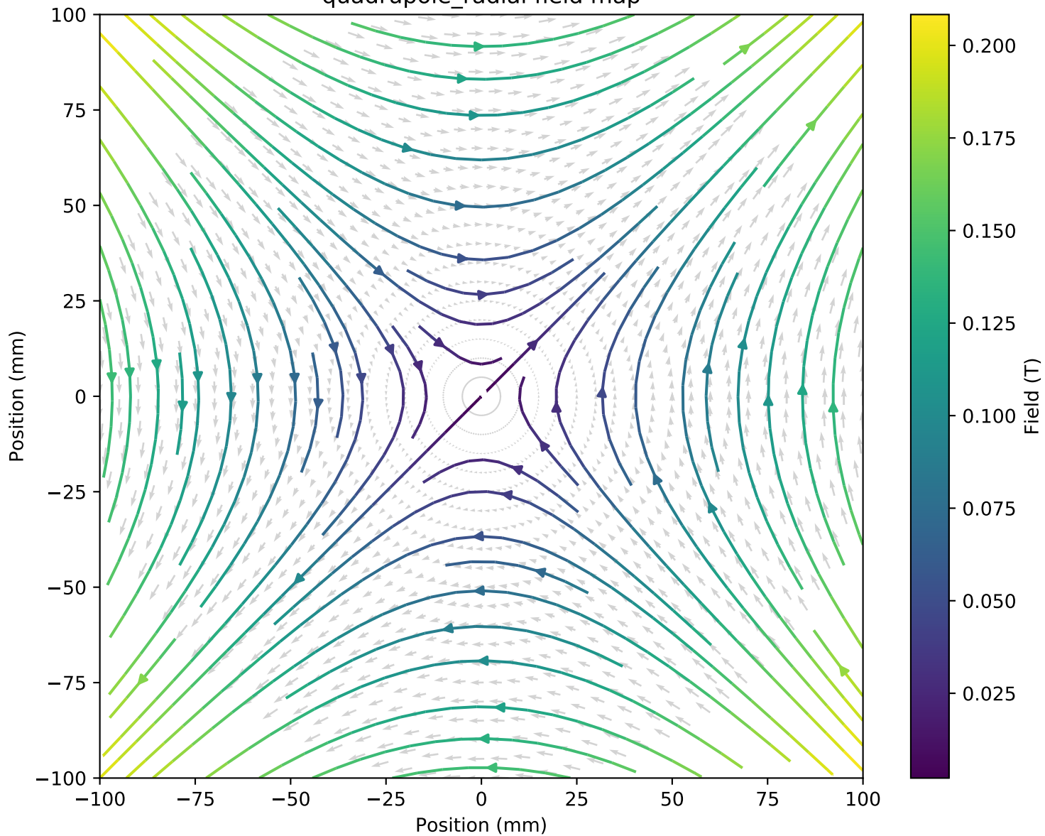
quadrupole_radial field map
