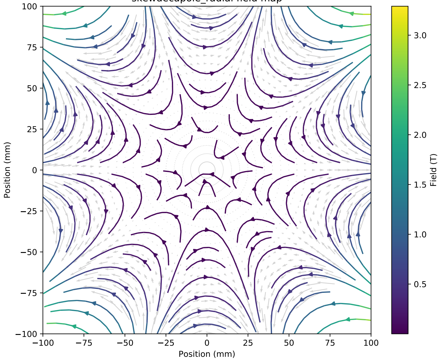
skewdecapole_radial field map
