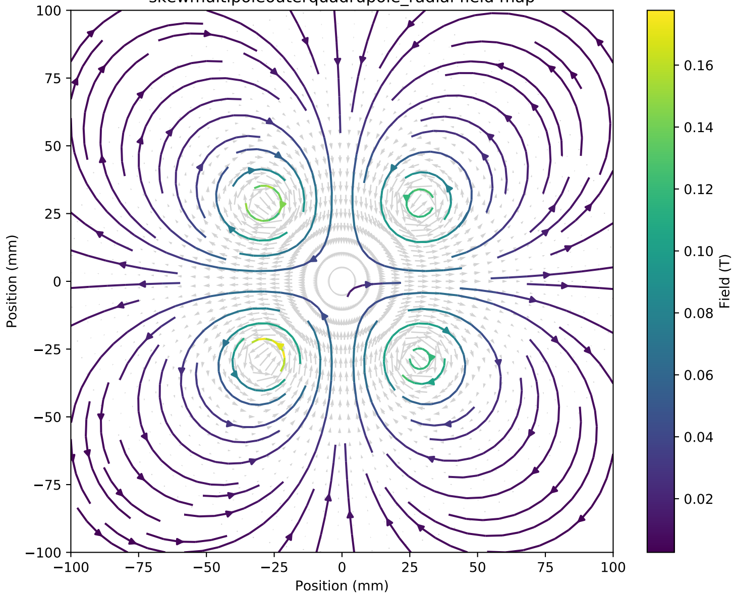
skewmultipoleouterquadrupole_radial field map
