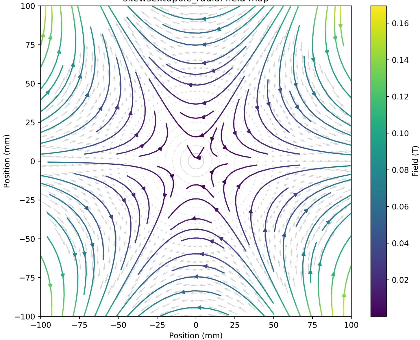
skewsextupole_radial field map
