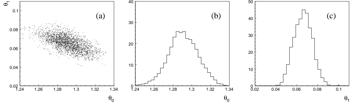
Fig. 3: MCMC marginalization of the posterior pdf p(\theta_0, \theta_1 | y) : (a) scatter-plot of points in (\theta_0, \theta_1) plane and the marginal distribution of (b) the parameter of interest \theta_0 and (c) the nuisance parameter \theta_1 .
