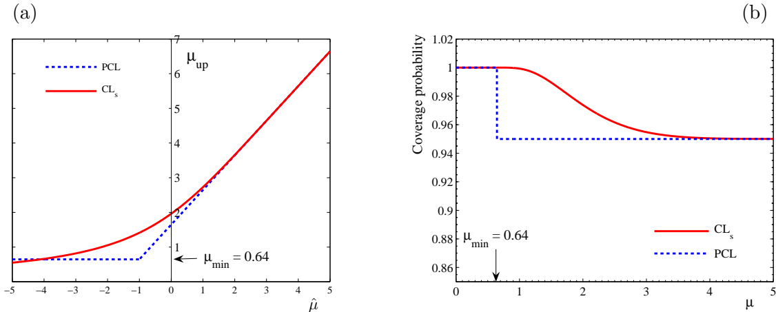
Figure 3: (a) Upper limits from the PCL (dashed) and \text{CL}_s (solid) procedures as a function of \hat{\mu} , which is assumed to follow a Gaussian distribution with unit standard deviation. (b) The coverage probabilities from the PCL (dashed) and \text{CL}_s (solid) procedures as a function of \mu .
