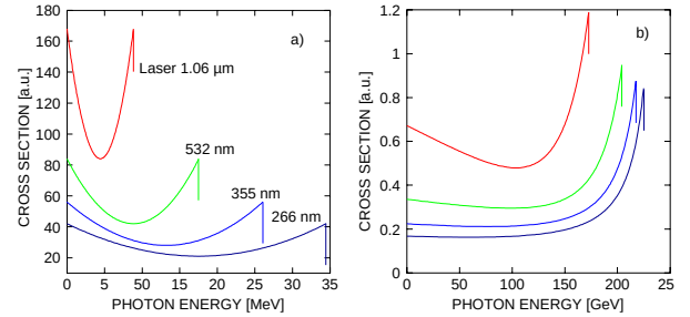
Figure 1: Compton cross section for the first four harmonics of an Nd:YAG laser scanning a 1 GeV (a) and 250 GeV (b) electron beam.
