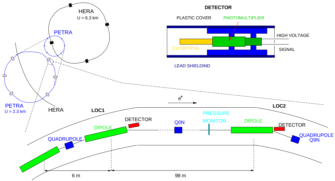
Figure 4: Schematic setup for background measurements at PETRA.
