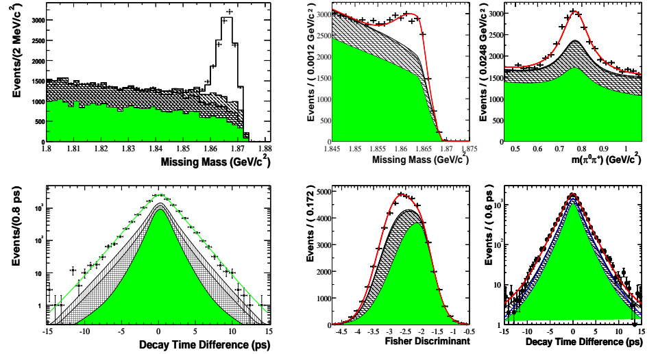
Fig. 3: Left: the missing mass (top) and \Delta t (bottom) distribution of B^0 \rightarrow D^{*\mp}\pi^\pm events. The \Delta t plot has been obtained after requiring m(\phi) > 1.860 GeV/c 2 . Right: the missing mass, \rho mass, Fisher discriminant and \Delta t distribution of B^0 \rightarrow D^{*\mp}\rho^\pm . The \Delta t plot has been obtained after requiring m(\phi) > 1.854 GeV/c 2 , 0.60 < m(\pi^+\pi^0) < 0.93 GeV/c 2 , and \mathcal{F}_D < -2.1 . In all plots, the result of the fit is superimposed on the data. The hatched, cross-hatched and shaded areas are the peaking B\bar{B} , combinatoric B\bar{B} and continuum background contributions, respectively.
