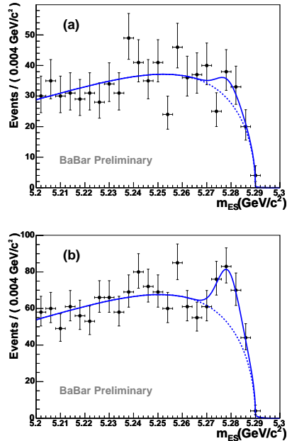
Figure 4. Fitted m_{ES} distribution for B^0 \rightarrow X^\pm K^\mp with the X^\pm signal region selection, |m(J/\psi \pi^\pm \pi^\mp) - 3872 \text{ MeV}/c^2| < 12 \text{ MeV}/c^2 , (a), and with the sideband region selection, 48 < |m(J/\psi \pi^\pm \pi^\mp) - 3872 \text{ MeV}/c^2| < 72 \text{ MeV}/c^2 , (b).
