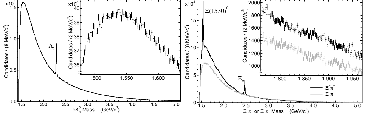
Figure 1: Invariant mass distributions found in the inclusive search for pentaquarks in e^+e^- collisions: pK_s^0 invariant mass (left) and of \Xi^-\pi (right). In the plot on the right distributions are shown for \Xi^-\pi^+ (black) and \Xi^-\pi^- (grey). The insets are magnification of the mass regions in which pentaquark states have been reported.
